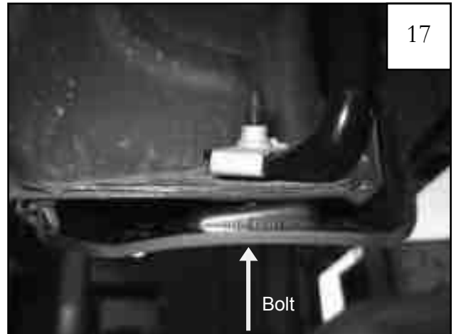
17 Thread 35 mm bolt through hole in forward underside of flare and through factory hole in sheet metal. See step 19.
