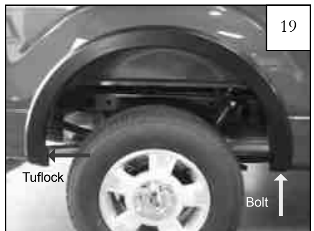
19 Using a 10 mm socket wrench, tighten 35 mm bolt through spacer and factory hole in sheet metal. Using a #2 Phillips driver, tighten the tuflock.
