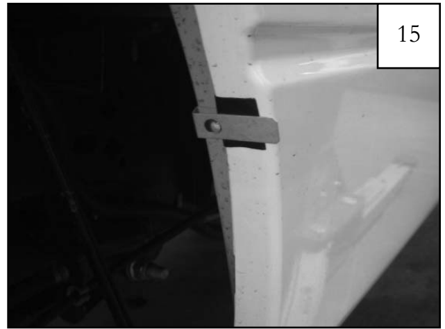
15 Install a long clip over each of the four black tabs placed on the sheet metal in Step 14.
