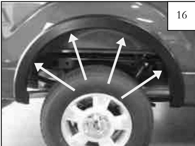
16 Hold flare to vehicle and start truss head screws through the two topmost holes in wheel well. Then start truss head screws through remaining two holes in flare. Tighten all screws.
