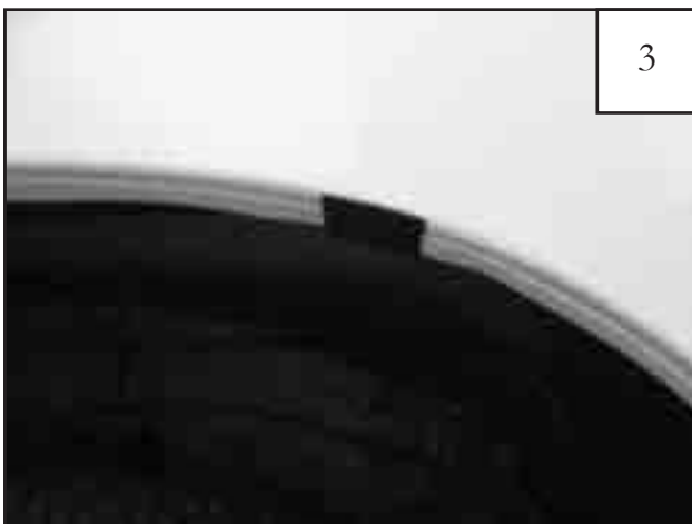
Remove flare from fender. Center a supplied black tab over each mark made in step 1.
