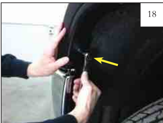
18 While holding Flare on vehicle, install factory screw removed in Step 7 through flare and into factory hole. Do not fully tighten at this time.
