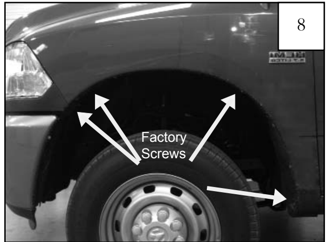
Remove four factory installed screws with 8 mm socket wrench.
