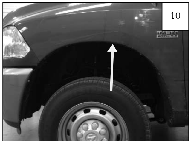
Install supplied clip (CL1-0022) at this location. See Steps 11, 12, 13, & 14.
