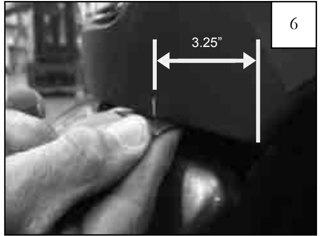
Measure 3.25" from wheel well along headlight mounting and mark with a grease pencil. Remove white backing from 1"x1.5" Black Tab. Center tab at mark, hook around lip, and install.
