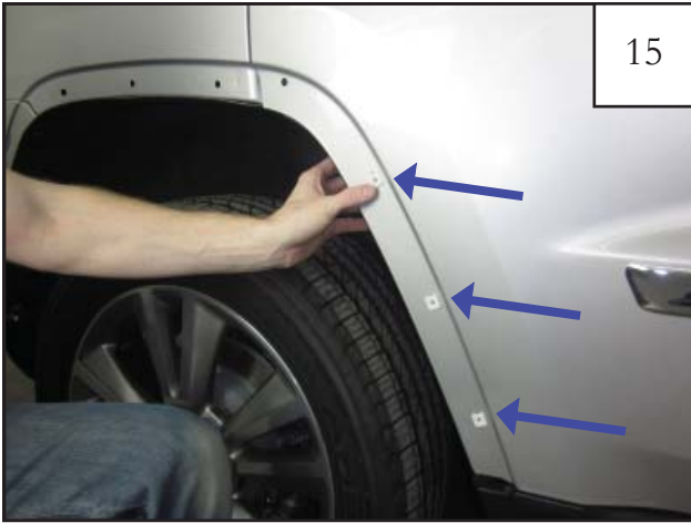
15 Install provided Grommets (GR1-0002) at the (3) locations indicated in image above.
