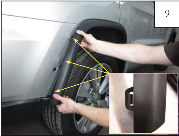
Starting at the end of the factory rear main flare, firmly grip part and pull to remove from vehicle. Note: You will hear popping sounds as the factory fasteners release from vehicle. This is normal. Use a pry tool to help release factory flare tabs from the rear bumper (see inset image).
