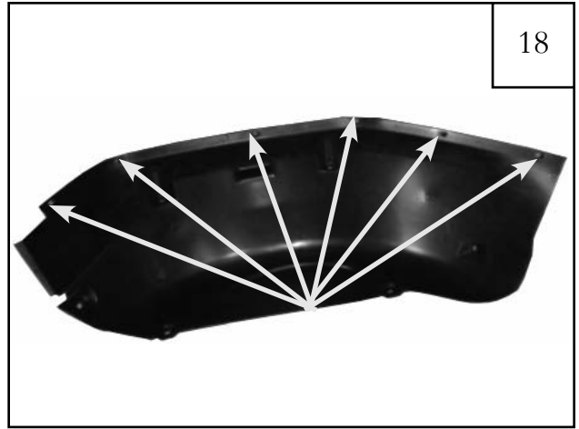
#14 U-Clip locations.
