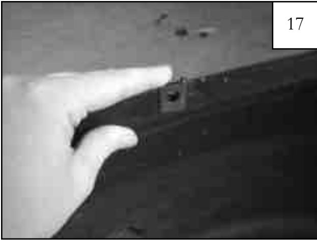
Install supplied #14 U-Clips over existing holes in splash shield (6 places). Flat side will be visible once splash shield is reinstalled.
