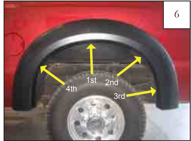
Position flare on fender and install screws through holes in flare and into clips with a #2 Phillips screwdriver in order shown. NOTE: If given order is not used, part is more difficult to install.
