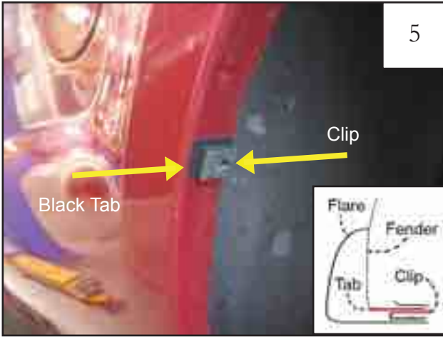
Install a clip over each of the black tabs installed in Step 4.
