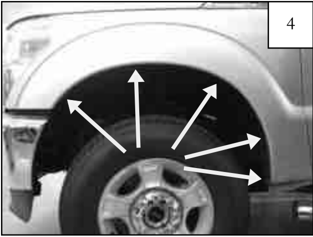
Remove five factory screws with a 7/32" socket wrench. Save screws for reinstallation.
