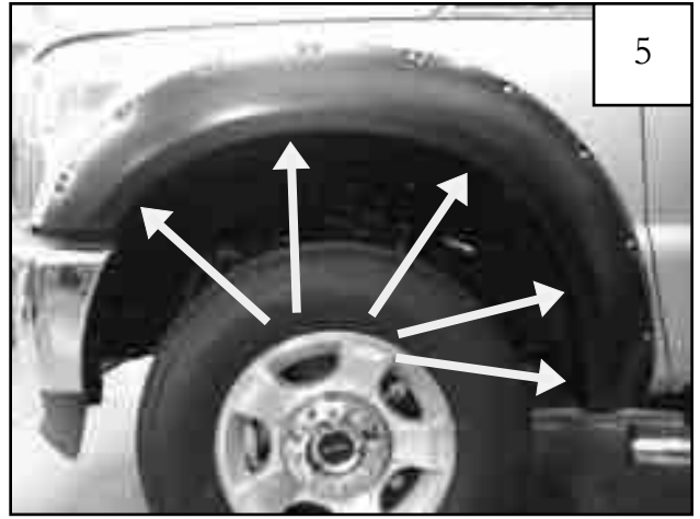
Position flare on fender, lining up factory holes and holes in the flare. Starting with the top, centermost screw, reinstall factory screws through holes in flare and fender with a 7/32" socket wrench.
