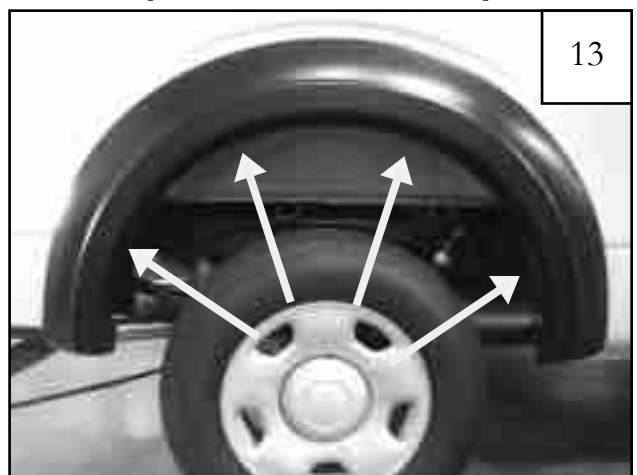
Hold flare to vehicle and mark the location with a grease pencil of the four holes in the flare. Note: Rear flares are similar enough that either will fit against the body of both sides. The wheel well hole locations will be wrong if the flare is on the wrong side. Driver's side flare is marked with an "L" and passenger's side flare is marked with an "R".
