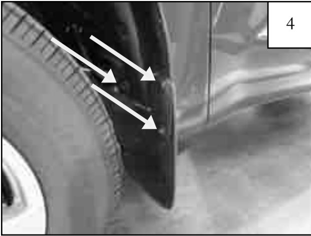
Remove three hex bolts from factory mud flap, using a 10mm socket.
