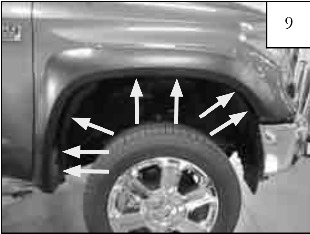
Ensure flare is properly positioned and tighten all screws. (Repeat for other side of vehicle) Installation Complete.
