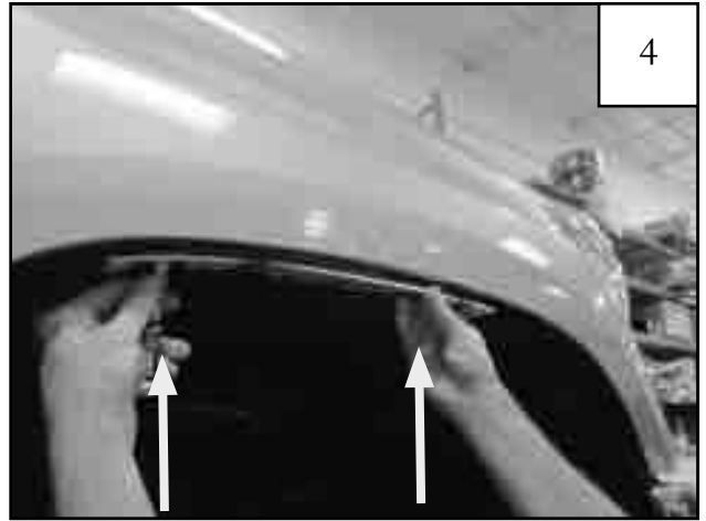
Using two supplied 20mm Hex Screws (SW1-0036), attach bracket to factory holes with a 10mm socket.
