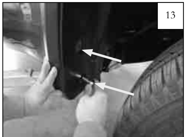
Start two supplied 20mm Hex Screws through the rearward most holes of flare and into the factory hole in fender.
