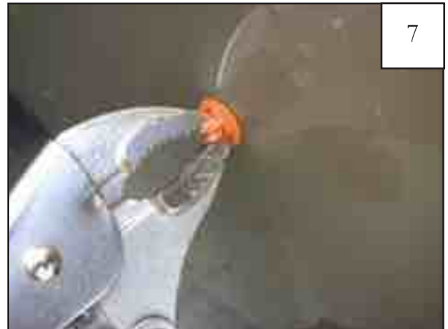
Remove three clips from fender using vise grips, pulling with a rocking motion. See step 8.
