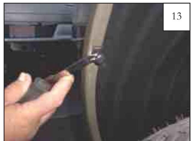
Remove plastic screw located at front of wheel well by turning clockwise 1/2 turn with a flat head screwdriver and prying out.
