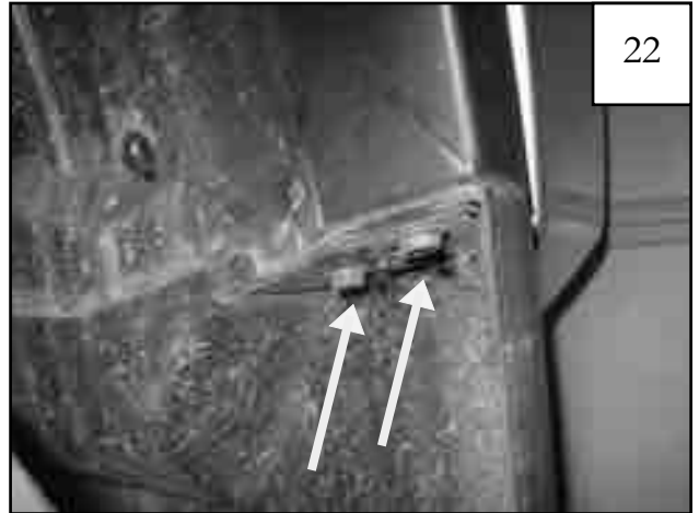
Remove two bolts from mud flap.
