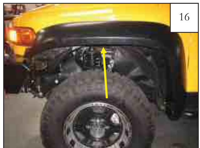
Install one supplied Christmas Tree Fastener in top hole. Check that edge trim is seated correctly, then tighten all bolts.
