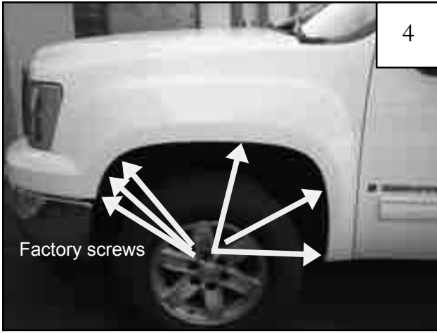
Using a 7mm socket, remove six factory screws from wheel well and save for reinstallation.
