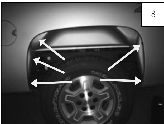
Slide a supplied Clip (CL1-0005) over lower five tabs. Clips may need to be adjusted to align with holes in flare.
