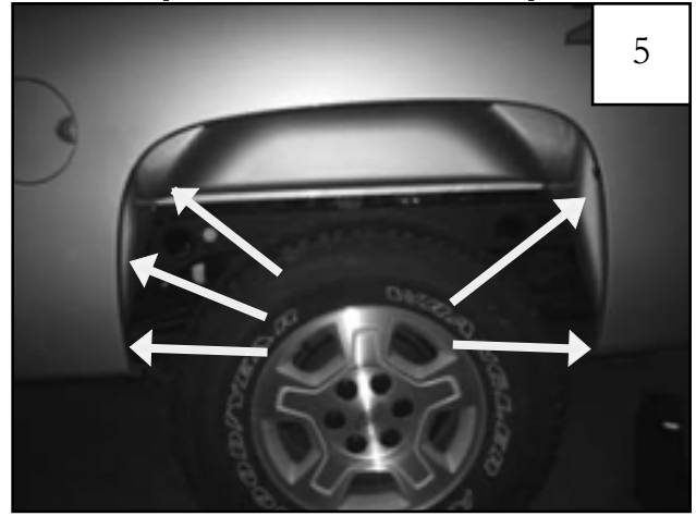
Five clip locations.
