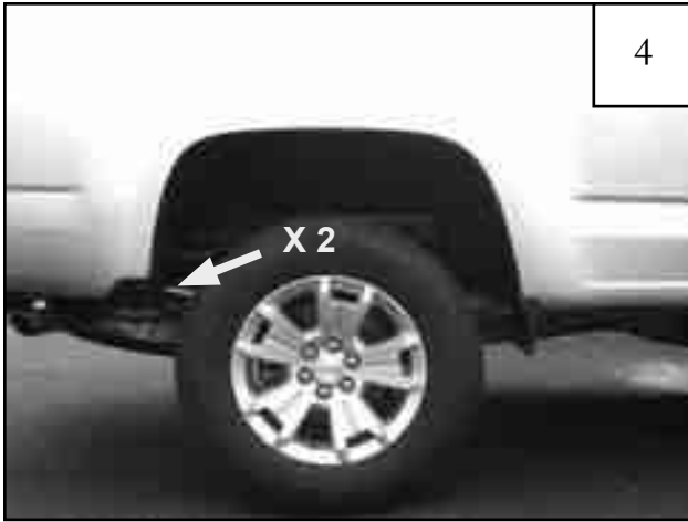
Using a T-15 torx bit, remove two factory fasteners from the mud guard in the lower rear of the wheel well. Discard factory fasteners only.
