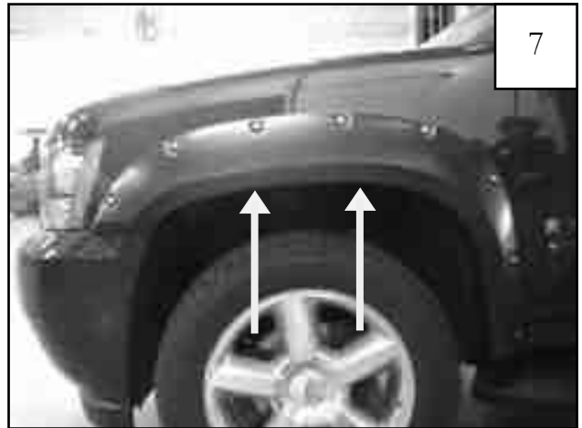
Retainer locations.
