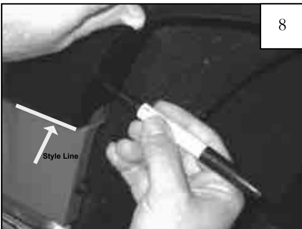
While holding the flare firmly in position, mark the remaining five hole locations with a grease pencil or sharpie, using the holes in the flare as a guide. Press inward firmly on the flare above each hole location before making each mark, this will ensure proper fit. See next step.
