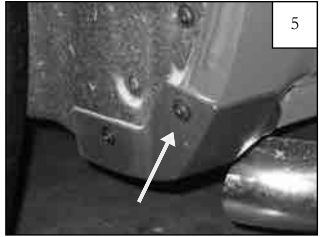
Using a T-15 Torx bit, remove two factory screws in mudguard at rear of front wheel well.
