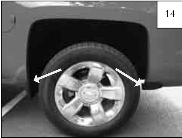
Using a T-15 Torx bit socket wrench, remove factory installed screws. Discard screws.
