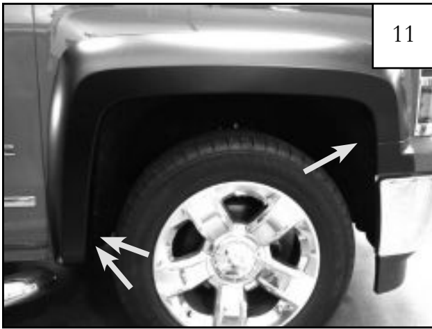
11 Locate flare into position on vehicle. Install supplied screw (SW1-0056) through two bottom rear holes in flare and into factory hole in front of wheel well.
