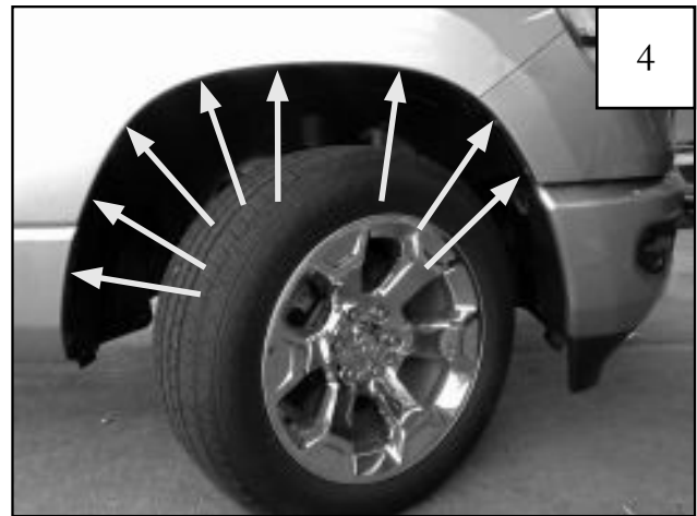
Remove and keep (8) factory installed screws. The remaining screws will be re-used to install the front flare.
