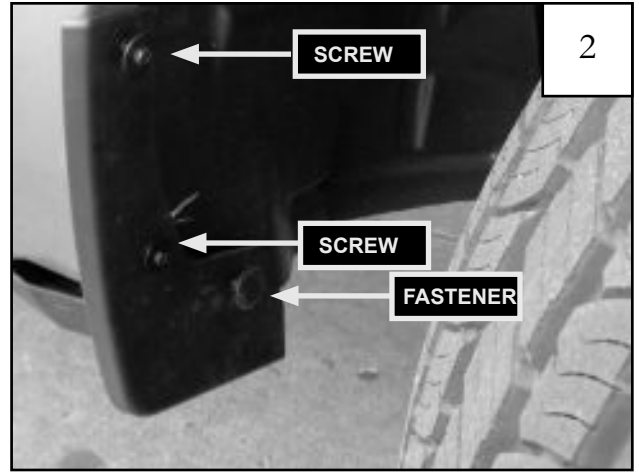
Remove (2) factory installed screws, and (1) factory installed fastener, and remove mud flap from vehicle.
