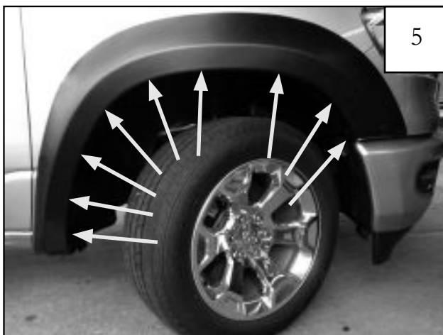
Hold flare to vehicle and start re-installing the remaining (9) factory screws with a 8mm socket. Do not tighten.
