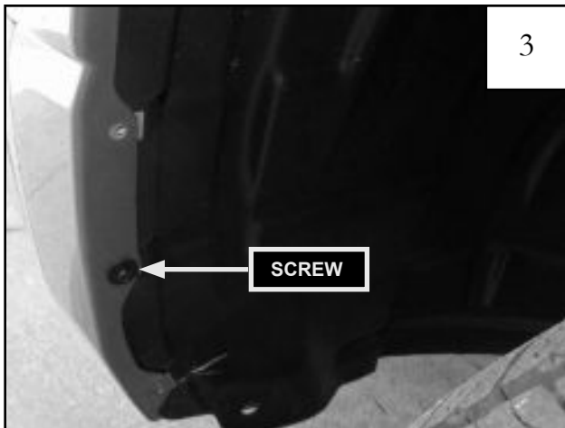
Re-install the previously removed lower factory screw as indicated above. Keep remaining screw. Fastener can be discarded.
