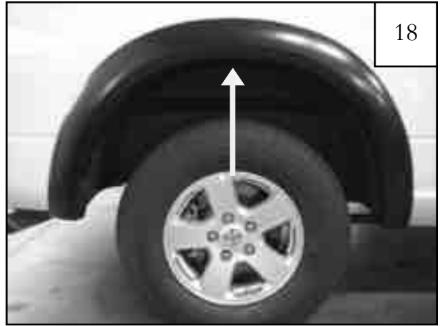
While holding flare onto vehicle, start a #8 x 3/4" Washer Panhead Screw using a Phillips screwdriver. Do not tighten.
