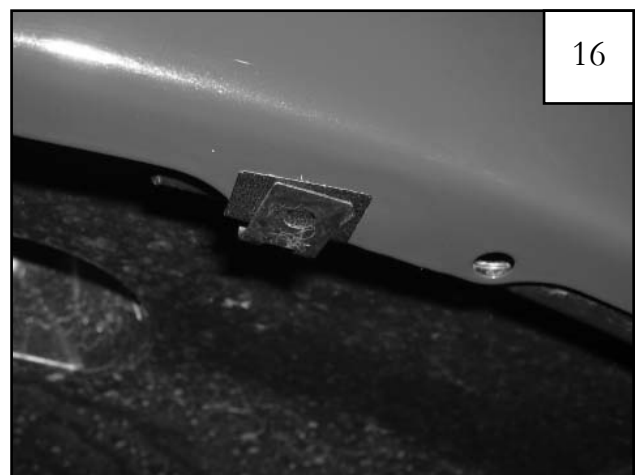
Install #10 U-Clip (CL1-0022) over tab and existing factory hole.
