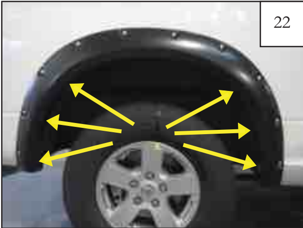
Hold flare in place while you start six supplied screws (SW1-0056) using a phillips screwdriver. Do not tighten.
