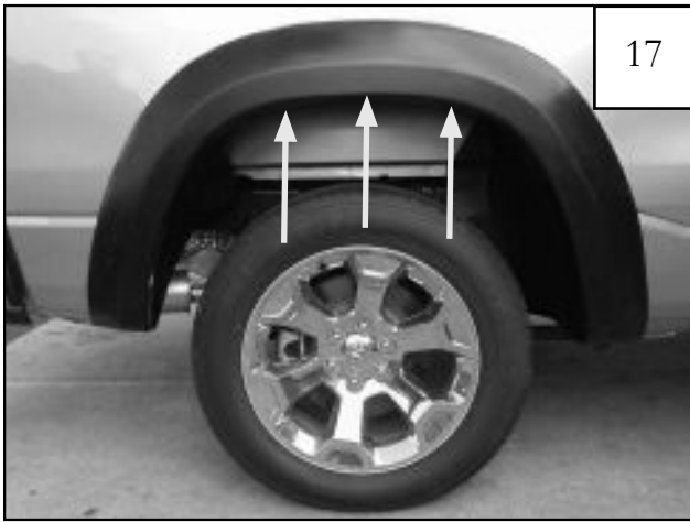
Hold flare in place and reinstall (3) factory screws removed in Step 16. Do not tighten.
