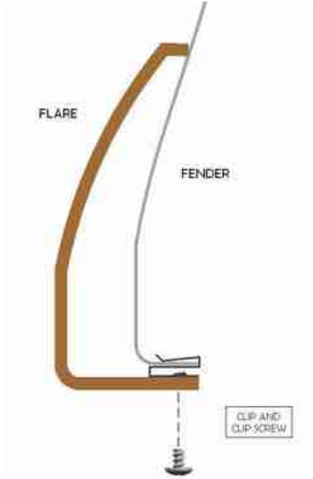
Illustration #2 Cross Section of Flare and Fender With Clip and Screw
