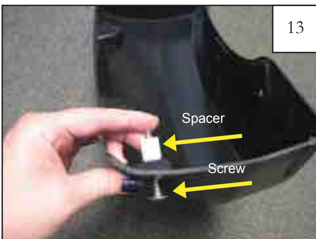
On the bottom of the door, pry out the fastener. Open access door. Remove edge protector from door lip and discard. Insert two plastic grommets into the square holes on the edge of the door and one into the fastener hole. Insert the supplied Screw (SW1-0034) through bottom hole in flare, and slide the supplied Spacer (SP1-0004) onto Screw on inside of flare
