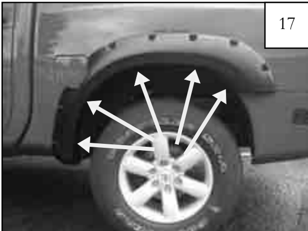
Driver Side Flare: Insuring the flare is properly located on fender, apply moderate pressure to outside surface of flare, and tighten screws, beginning with the lower front screw working toward the access door.
