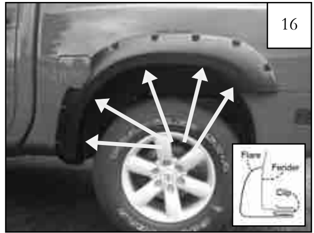
Driver Side Flare: Install five Clips (CL1-0005) over fender lip, lining up the hole in clips with the holes in flare. Start Screws (SW1-0050) in each Clip. Do not fully tighten screws.
