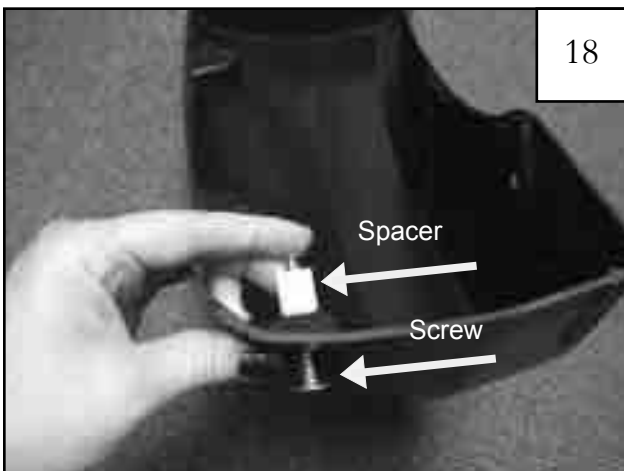
On the bottom of the door, pry out the Christmas Tree fastener. Open access door. Remove edge protector from door lip and discard. Insert two plastic grommets into the square holes on the edge of the door and one into the Christmas tree hole. Insert the supplied Screw (SW1-0034) through bottom hole in flare, and slide the supplied Spacer (SP1-0004) onto Screw on inside of flare
